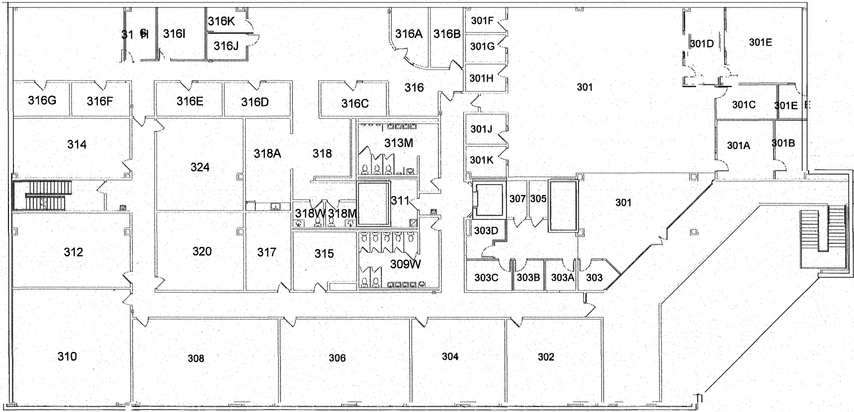
① HACC - THIRD FLOOR 1/16" = 1'-0"
